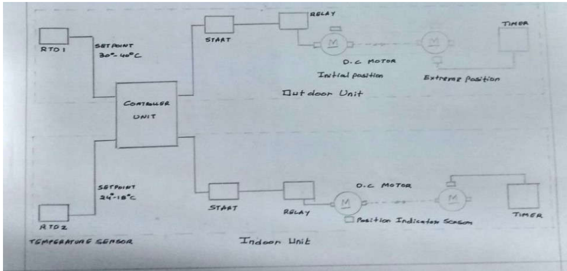
FIGURE 1 Block Diagram of the above project
